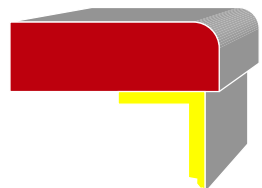
Polished cut-out for under-mount sink with R8 or A30 upper edge
